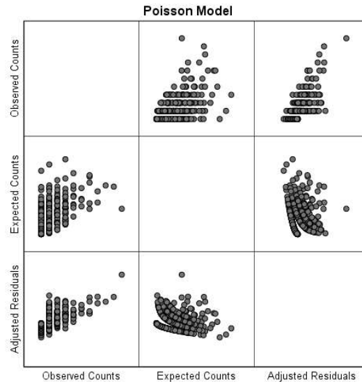
Figure 2: Poisson Regression Analysis
